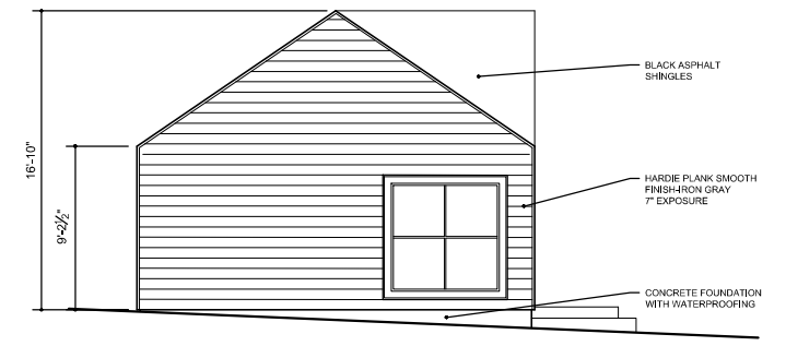
OPTION 2 - SOUTH ELEVATION
