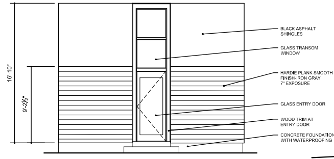
OPTION 2 - EAST ELEVATION
