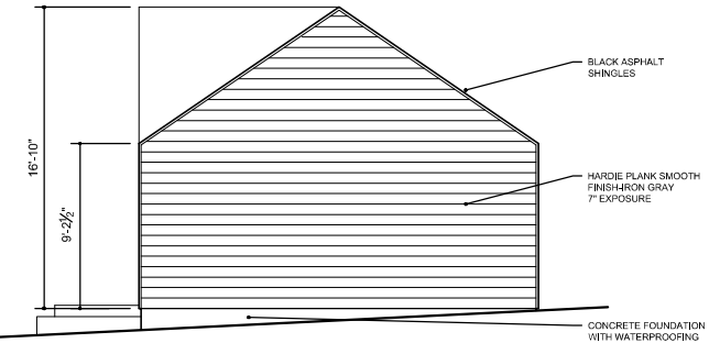
OPTION 2 - NORTH ELEVATION
